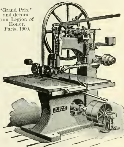
NO. 110, SELF FEED RIP SAW.
